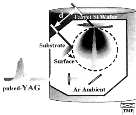
FIG. 1. A schematic of the laser ablation instrument.
