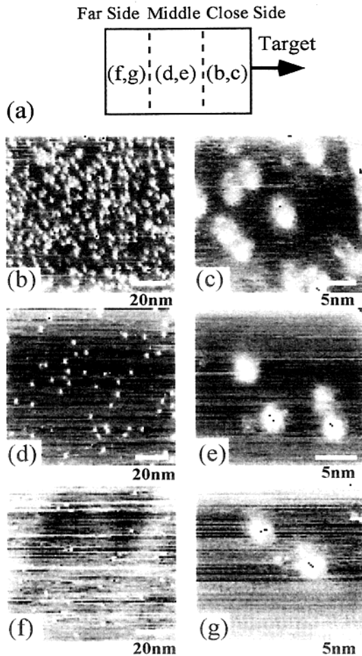
FIG. 3. A set of STM images taken at different locations of the HOPG substrate (both sides and the middle) as indicated in the schematic in (a).
