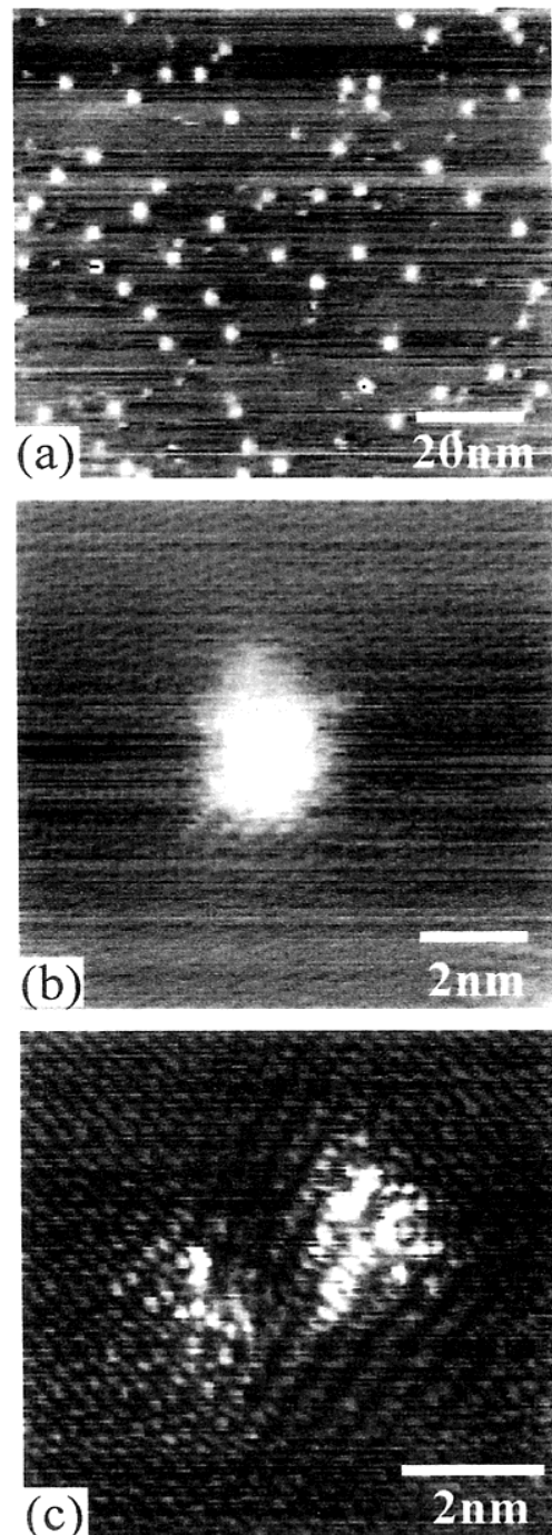
FIG. 2. (a) A typical STM image of the Si nanoparticles deposited on HOPG. (b) A high resolution STM image showing the details of the surface morphology. (c) A Si nanoparticle surrounded by a superlattice structure.
