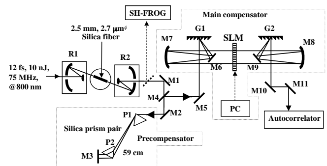
Fig. 1. Layout of the experimental setup. M1–6, M9–11, silver-coated plane mirrors; M7 and M8, silver-coated spherical mirrors, R = 400 mm; P1, P2, Brewster-angle cut silica prisms; G1, G2, gold-coated gratings d = 300 lines/mm; R1, R2, reflective objectives (36 \times ); SLM, spatial light modulator controlled by computer (PC).
